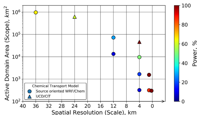
Figure 6. Power of detecting a 0.5 µg/m³ maximum exposure disparity between groups for each combination of spatial resolution and domain scope, including both source oriented WRF/Chem (dot) and UCD/CIT (triangle) CTM results. A power of 90% indicates that there is a 90% probability of correctly concluding that exposures are different between the groups.
